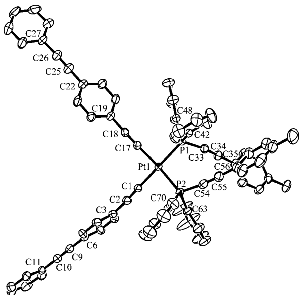
Figure 1. Molecular structure of cis -[Pt(C≡CC 6 H 4 C≡CPh) 2 -(PPh 2 C≡Ctol) 2 ] ( 2 ). Ellipsoids are drawn at the 50% probability level. Hydrogen atoms have been omitted for clarity.
