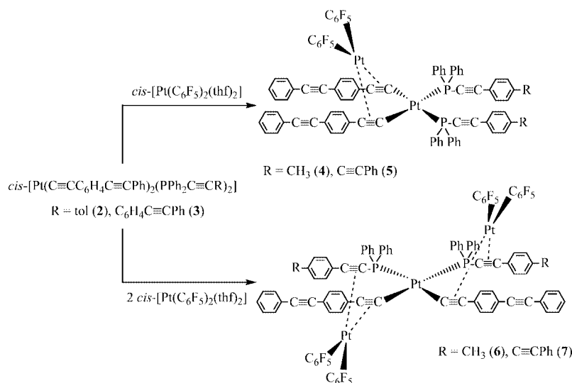
Scheme 1. Synthesis of complexes 4–7.
