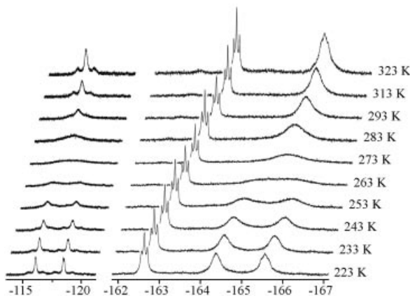
Figure 2. Variable-temperature ^{19}\text{F} NMR spectra (chemical shifts in ppm) of cis -[Pt(PPh 2 C≡CC 6 H 4 C≡CPh) 2 (μ-η 1 :η 2 -C α ,C β -C≡CC 6 H 4 C≡CPh) 2 ]Pt(C 6 F 5 ) 2 ( 5 ) in CDCl 3 .
