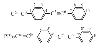
Figure 3. Labelling scheme for the carbon atoms in the ethynyltolan and (ethynyltolan)diphenylphosphane ligand.
